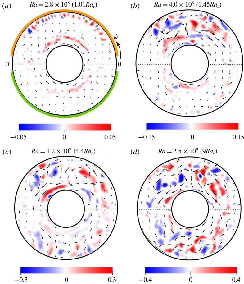
FIGURE 7. Plots of the measured horizontal velocity vectors (arrows) superposed on shaded contours of the z vorticity ( \text{s}^{-1} ) on a horizontal ( r, \phi ) plane at z = 170 mm for the onefold heterogeneous heat flux pattern ( q^* \approx 0.7 ). The boundary heat flux in the sector \phi = [0, \pi] is higher than the mean value. The plots are averaged over a run time of 360 s. The onefold boundary heat flux pattern is indicated in panel (a), with the orange (green) outline showing higher (lower) heat flux than the average. The values of Re_{peak} , Re_{rms} , Pe_{peak} and Pe_{rms} , in that order, are as follows: (a) 72, 20, 477, 131; (b) 98, 36, 648, 242; (c) 180, 76, 1194, 502; and (d) 216, 116, 1431, 773. The maximum velocity denoted by the longest arrow is 7.5 \times 10^{-4} \text{ m s}^{-1} , 1 \times 10^{-3} \text{ m s}^{-1} , 1.9 \times 10^{-3} \text{ m s}^{-1} and 2.2 \times 10^{-3} \text{ m s}^{-1} for (a), (b), (c) and (d), respectively.
