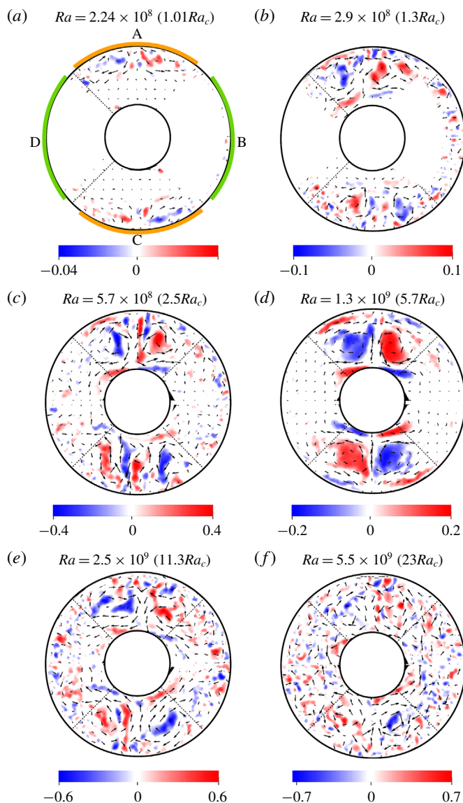
FIGURE 10. Plots of the measured horizontal velocity vectors (arrows) superposed on shaded contours of the z vorticity ( \text{s}^{-1} ) on a horizontal (r, \phi) plane at z = 180 mm for the twofold heterogeneous heat flux pattern ( q^* \approx 1 ) at progressively increasing Ra . The plots are averaged over a run time of 360 s. The twofold pattern is indicated in (a) with the orange (green) outline showing higher (lower) heat flux than the average. The values of Re_{peak} , Re_{rms} , Pe_{peak} and Pe_{rms} are, in that order, as follows: (a) 83, 26, 550, 169; (b) 132, 50, 875, 331; (c) 178, 84, 1179, 559; (d) 206, 106, 1370, 704; (e) 220, 128, 1460, 847; and (f) 226, 147, 1502, 976. The maximum velocity denoted by the longest arrow is 8.6 \times 10^{-4} \text{ m s}^{-1} , 1.4 \times 10^{-3} \text{ m s}^{-1} , 1.8 \times 10^{-3} \text{ m s}^{-1} , 2.1 \times 10^{-3} \text{ m s}^{-1} , 2.3 \times 10^{-3} \text{ m s}^{-1} and 2.4 \times 10^{-3} \text{ m s}^{-1} for plots (a)–(f), respectively.
