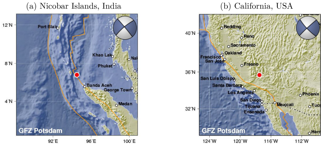
Figure 4. Two strike-slip earthquakes that are analysed in this paper. Major faults in the region are delineated by orange curves, and moment tensor solutions are inserted. Courtesy: GEOFON Program Hanka & Kind (1994), GFZ Potsdam.
