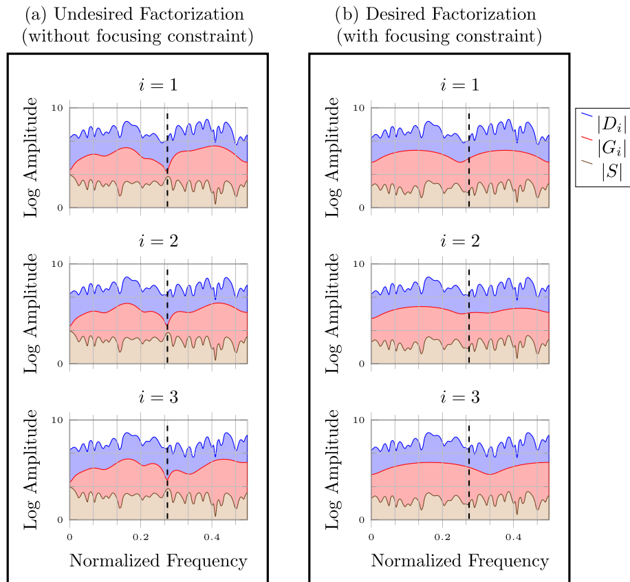
Figure 2. Two possible factorizations of the recorded spectra |D_i| , associated with the solutions of the IBD problem in eq. (4). In each of the plots the recorded spectrum is satisfied, that is, \log |D_i| = \log |G_i| + \log |S| as implied by eq. (3). In factorization (a), the estimated spectra associated with the path effects |G_i| are similar to each other for different i , for example, they have a common notch at the frequency indicated by the dashed line. Therefore, factorization (a) is physically unreasonable, provided that the receivers are separated by distances much larger than the wavelength. The focusing constraint in FBD obtains the factorization (b) that exactly matches the true factors—note that the |G_i| in this factorization are not only more white but also more dissimilar to each other.
