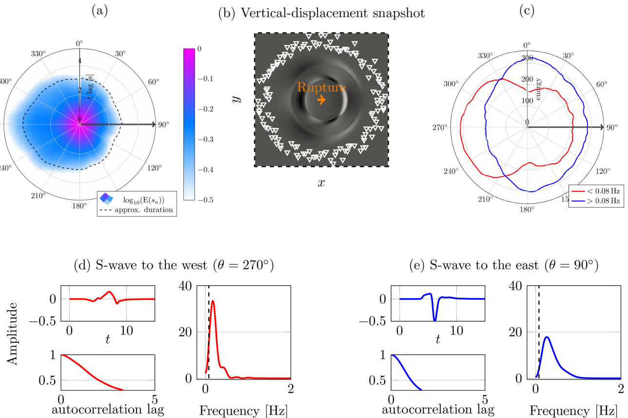
Figure 3. A synthetic experiment. (a) The envelope E(\hat{s}_a(t; \theta)) of the FBD-estimated auto-correlated source pulse is plotted (colour) as a function of the lag time (radius) and azimuth. The dashed curve indicates the source-pulse duration after smoothing along \theta . (b) Vertical displacement due to a rupture, coloured in grey scale as a function of the horizontal x and vertical y spatial coordinates, before the P and S waves are scattered by the boundaries (dashed lines) of the medium. Only receiver positions with r > 25 are marked by white triangles in order not to obscure the wavefield. (c) The energy of the FBD-estimated source spectrum, in both the low (red) and high (blue) frequency bands, is plotted to depict the redshift. In order to validate the FBD results, the direct S -wave pulse on the opposite sides of the rupture (see the text) is plotted in (d) and (e), respectively. The dashed vertical line separates the two frequency bands of (c).
