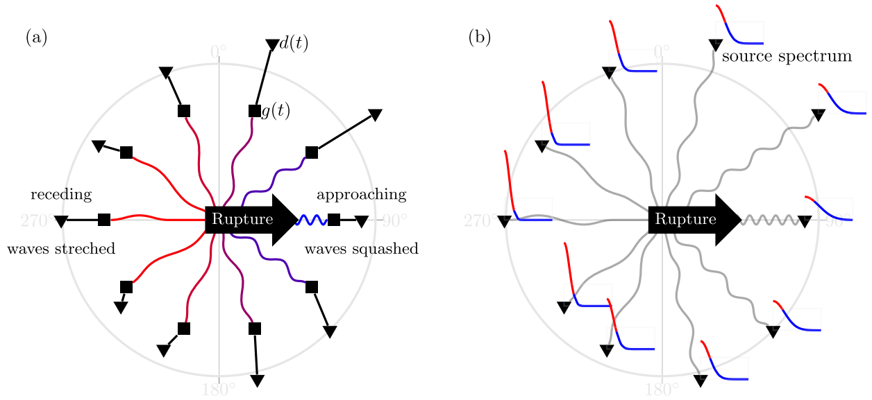
Figure 1. Schematic of waves emitted due to a rupture propagating from west (azimuth \theta = 270^\circ ) to east ( 90^\circ ). (a) Blue waves emitted towards the east are shortened, while the red waves travelling towards the west are lengthened. These waves undergo complex scattering (squares) before they reach the receivers (triangles), resulting in a challenging source-spectrum estimation problem. (b) FBD factorizes the measurements, effectively removes the complex scattering or path effects and directly estimates the source spectra (red-blue graphs) at the receivers. The variability of the normalized source spectrum with \theta can be used to infer the kinematic rupture parameters.
