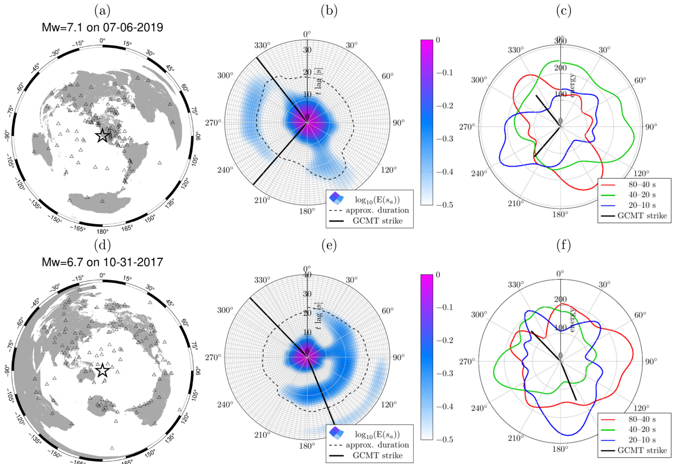
Figure 7. As in Fig. 3, except that the FBD results indicate complex rupturing. Redshift due to a unilateral rupture propagation cannot be identified during the analysis of these earthquakes, which are listed in the Table 1.
