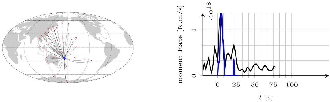
Figure B1. FBD estimated P -wave ASTFs for five different earthquakes with magnitudes 6.5 < M_w < 9.0 are plotted in black. For comparison, the ASTFs estimated using the SCARDEC method (Vallée et al. 2011) are plotted in blue. GSN stations are plotted in red.
